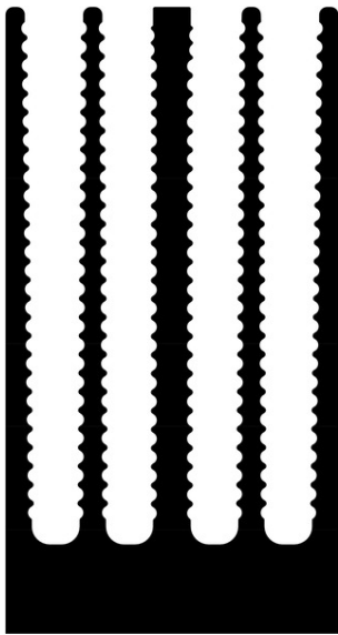
Profile heatsinks and fluid coolers>Standard extruded heatsinks 45 x 85 mm
